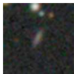
PGC 3501310 – Mag 17.78
